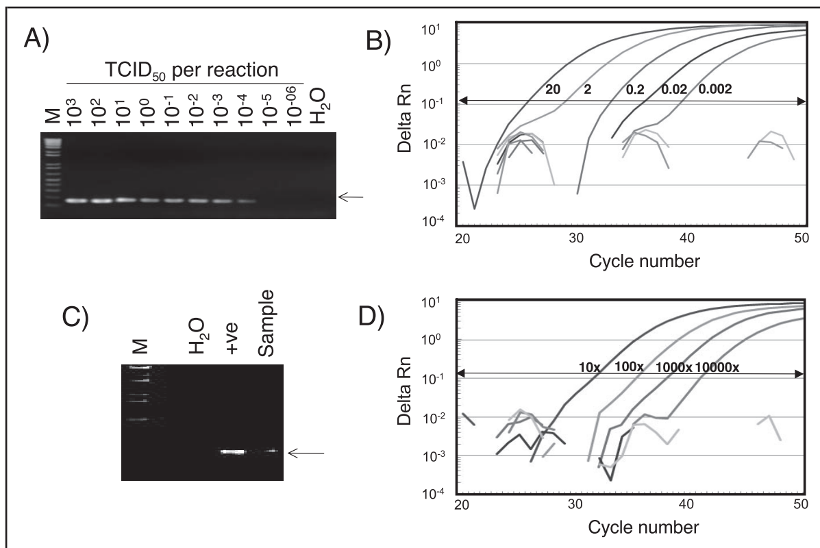
Fig. 1. Molecular detection of the novel H1N1 influenza virus by conventional and real-time RT-PCR assays.
